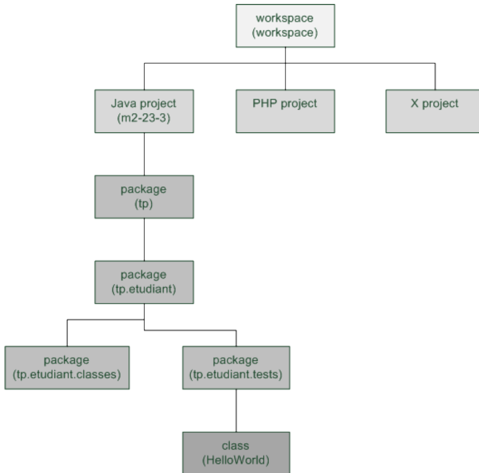
Figure 2.1. Workspace
